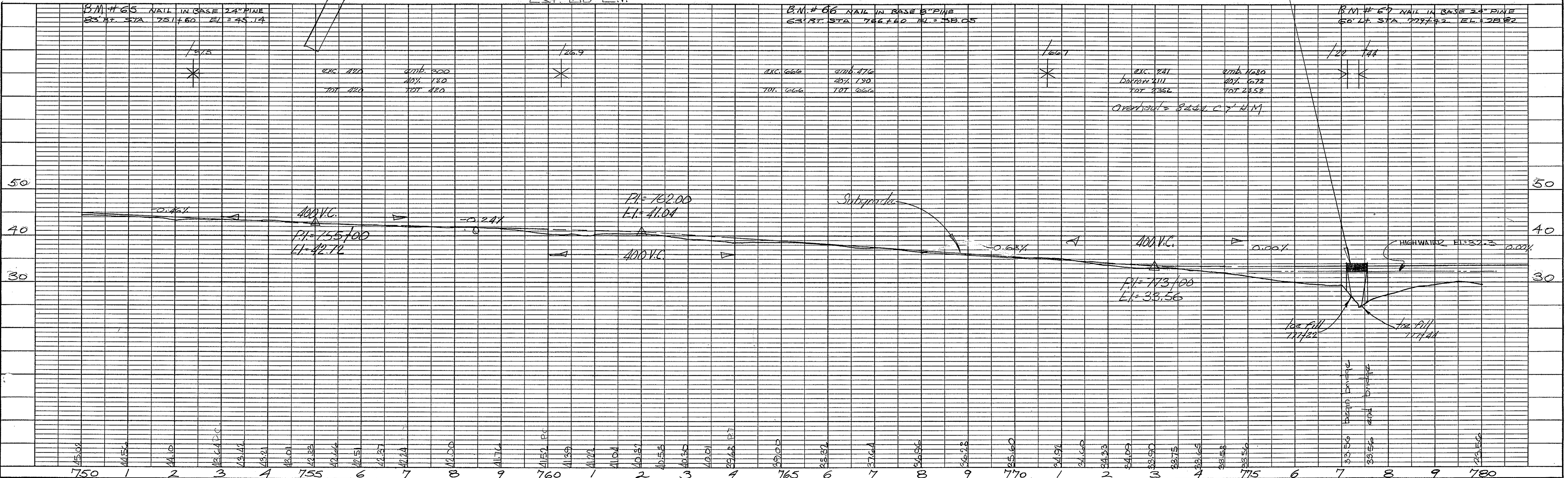
PLATE 1, PLAN-PROFILE KEUFER & ESSER CO.
